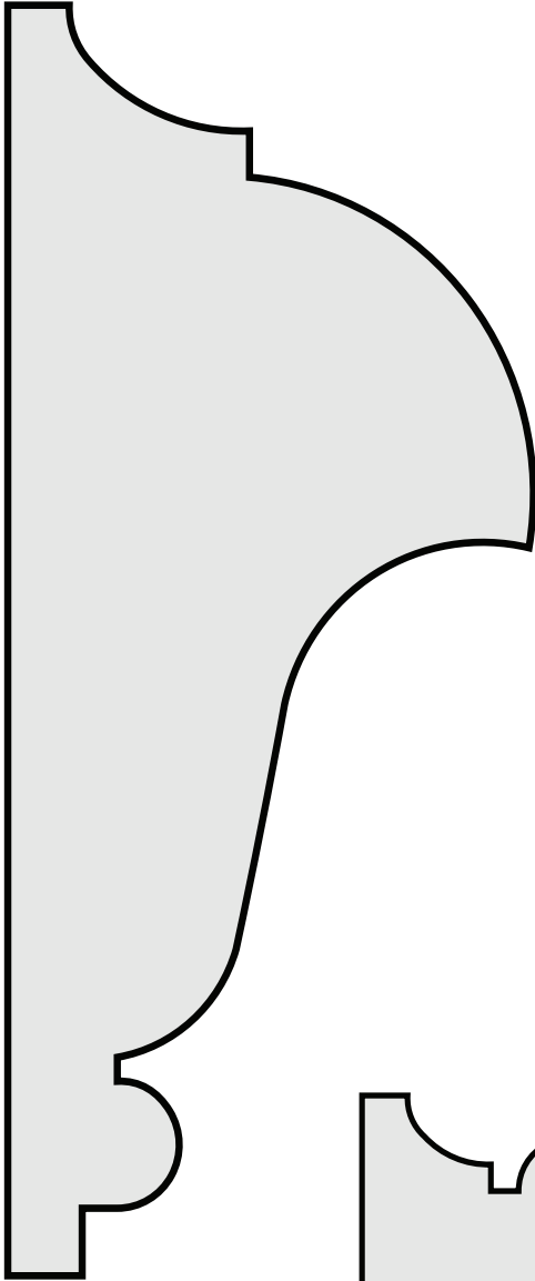
P77 2 1/2" x 6" PANEL MOULD
