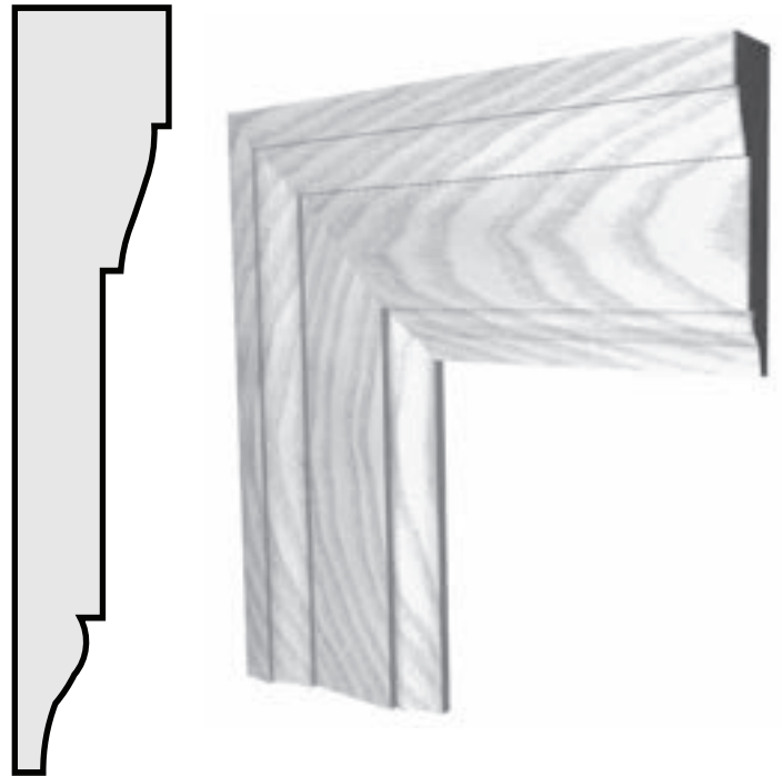
P167 3/4" x 3 5/16" CASING
