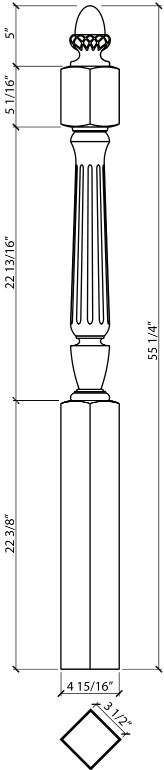
PNF503 3 1/2" x 55 1/4" COMBINATION NEWEL
