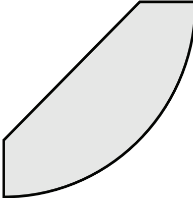
P24 1" x 2 13/16" (2" x 2" - 2" RADIUS) SEGMENT ROUND
