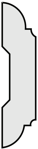
P176 5/8" x 2 9/16" CHAIR RAIL MOULD
