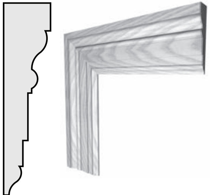
P169 7/8" x 3 1/2" CASING
