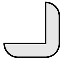
P247 1/2" x 1" FRIEZE MOULD
