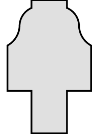
P294 1 3/8" x 7/8" SASH MUNTIN
