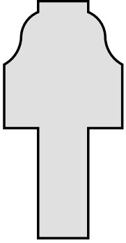
P291 1 3/4" x 7/8" SASH MUNTIN
