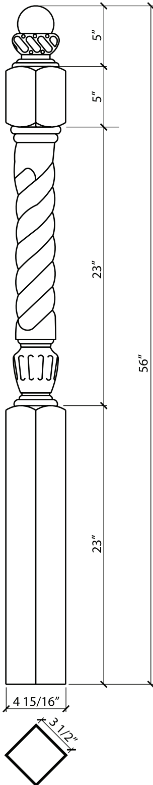
PNT701 3 1/2" x 56" COMBINATION NEWEL
