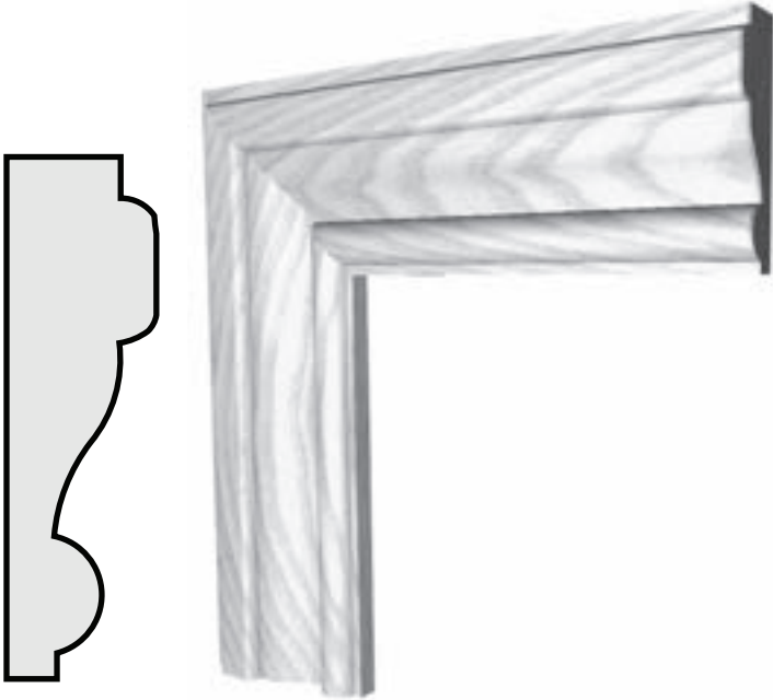
P160 3/4" x 2 1/2" CASING
