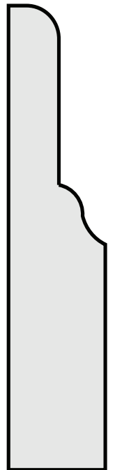
P61 3/4" x 3 1/2" BASEBOARD MOULD
