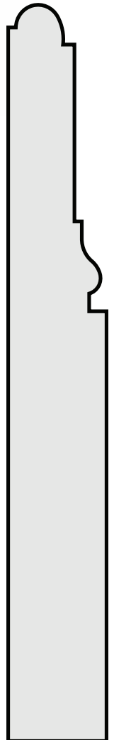
P70 3/4" x 5 7/16" BASEBOARD MOULD
