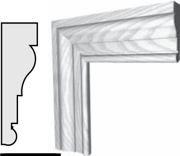
P166 3/4" x 2 1/2" CASING
