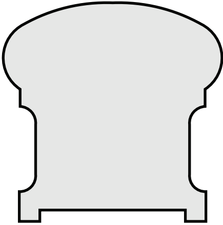
P202 2 1/4" x 2 1/4" HANDRAIL
