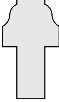
P222 1 3/4" x 1" SASH MOULD
