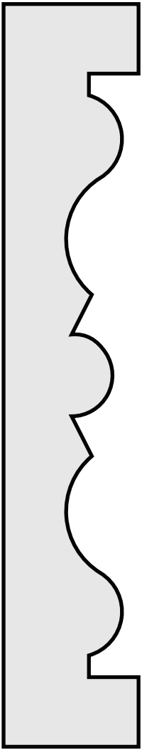
P154 1" x 5 7/16" CASING
