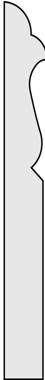
P71 3/4" x 6 7/16" BASEBOARD MOULD
