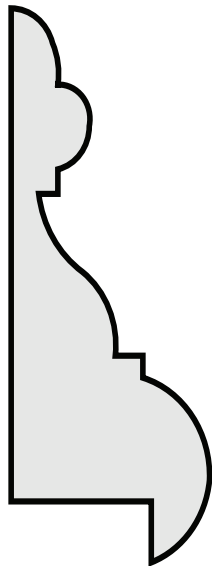
P135 1 1/16" x 1 11/16" RAISED PANEL MOULD
