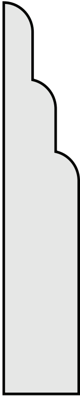
P60 13/16" x 4 1/8" BASEBOARD MOULD
