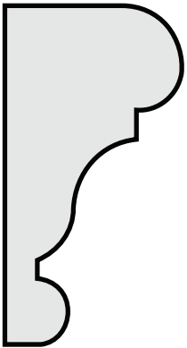
P275 1 1/16" x 2" PANEL MOULD
