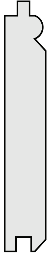
P219 3/4" x 4 5/16" STANDARD SIDING
