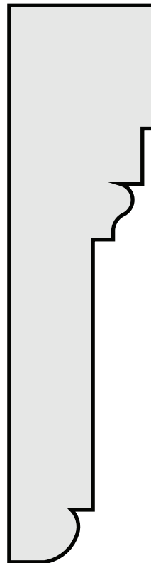
P159 1 1/16" x 4 1/8" CASING
