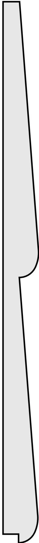
P208 5/8" x 9 3/4" STANDARD SIDING
