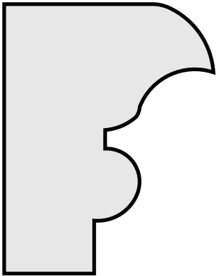
P105 1 1/8" x 1 5/8" PANEL MOULD
