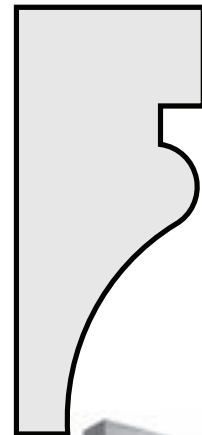
P93 1 1/16" x 1 1/2" PANEL MOULD
