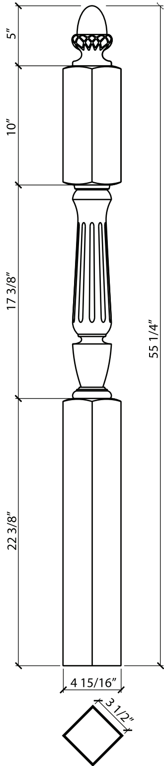
PNF504 3 1/2" x 55 1/4" LANDING NEWEL
