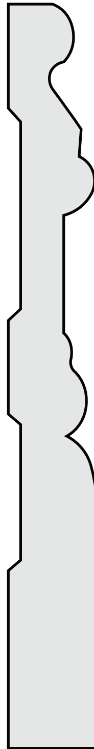
P289 15/16" x 7 9/16" BASEBOARD MOULD
