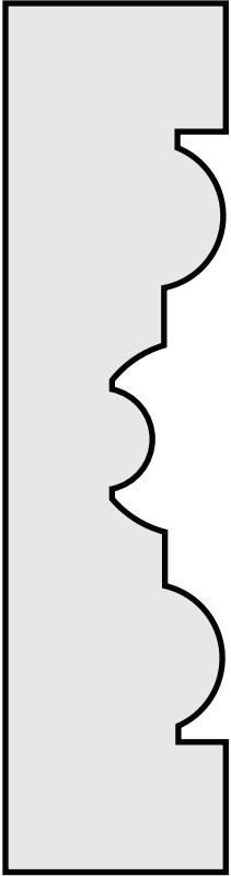
P158 1 1/16" x 4 1/8" CASING
