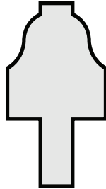
E 1 3/8" x 3/4" SASH MUNTIN (ALSO AVAILABLE IN BALSA)
