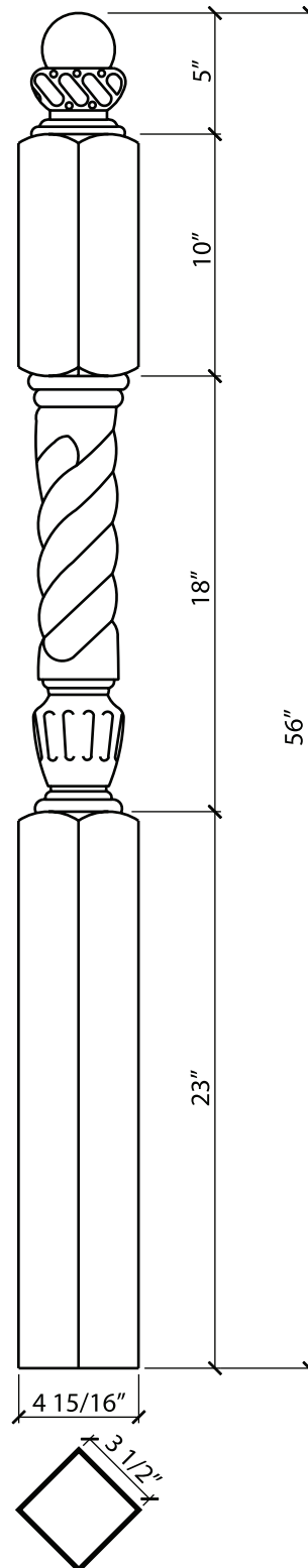
PNT702 3 1/2" x 56" LANDING NEWEL
