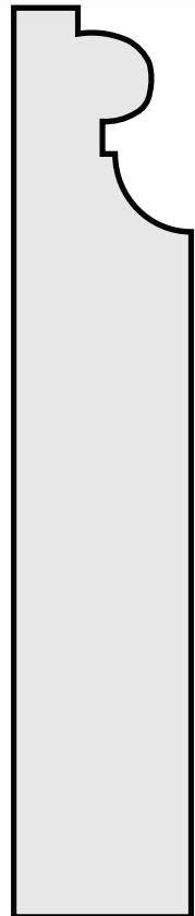
P57 7/8" x 4 3/8" BASEBOARD MOULD
