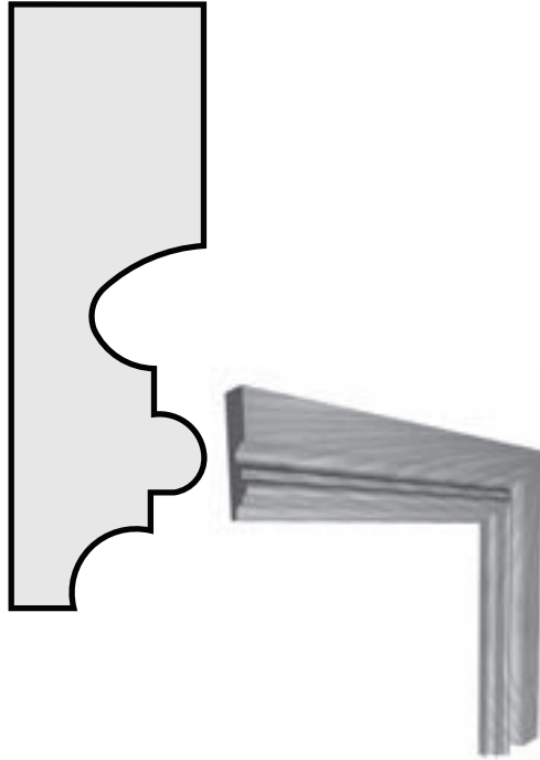
P80 15/16" x 2 7/8" PANEL MOULD
