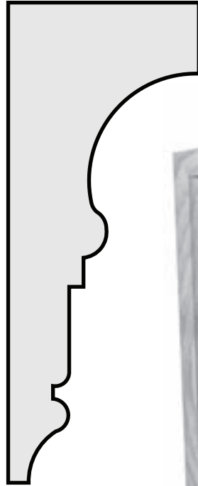
P165 1 7/16" x 3 1/2" CASING
