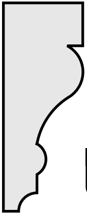
P40 1 3/16" x 2 1/8" FRIEZE MOULD
