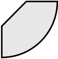
P22 11/16" x 1 7/16" (1" x 1" - 1" RADIUS) SEGMENT ROUND
