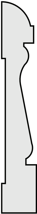
P58 3/4" x 4 3/8" BASEBOARD MOULD
