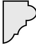
P75 3/4" x 15/16" PANEL MOULD
