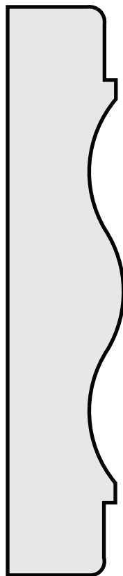
P157 13/16" x 4 1/4" CASING
