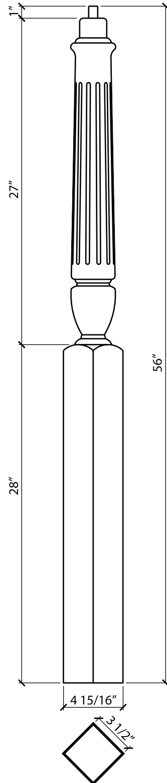
PNF502 3 1/2" x 56" LANDING NEWEL
