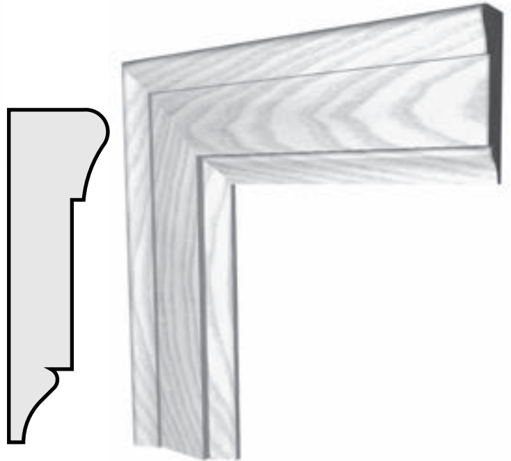
P162 3/4" x 2 1/2" CASING
