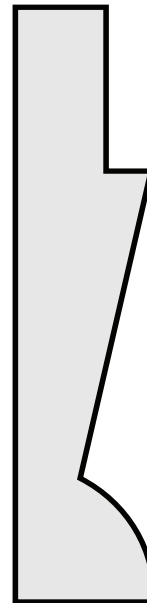
P130 1 1/2" x 2 1/4" RAISED PANEL MOULD
