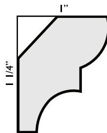
P257 3/4" x 1 9/16" CROWN/CORNICE
