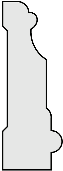
P65 1 1/4" x 3 1/2" BASEBOARD MOULD
