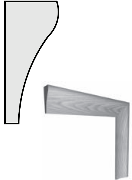
P81 1" x 2 1/4" PANEL MOULD
