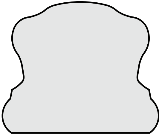
P8000 2 3/4" x 2 5/16" HANDRAIL
