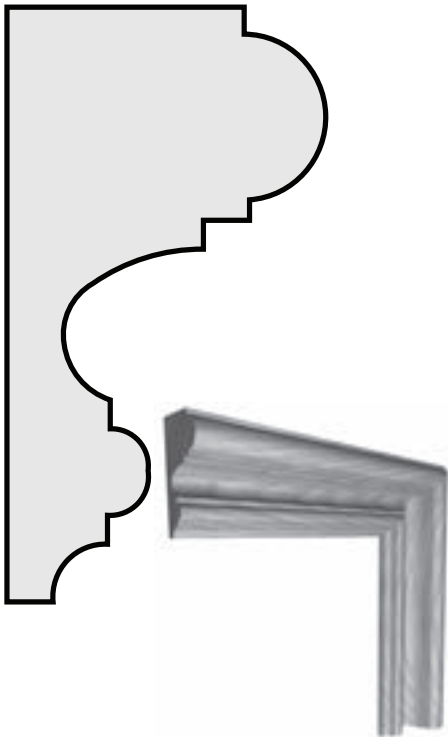
P82 1 11/16" x 3 1/8" PANEL MOULD
