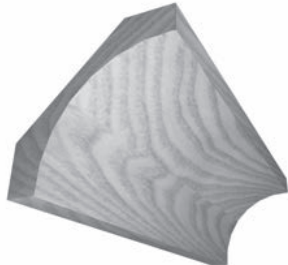
P144 1 \frac{3}{8}'' x 4 \frac{7}{8}'' COVE MOULD
