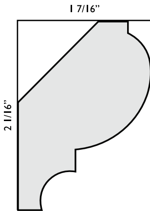
P266 1" x 2 1/16" COLUMN CAP/BASE
