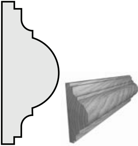
P32 1" x 2 1/2" ASTRAGAL
